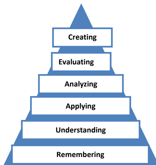
Figure 2. Taxonomy level
